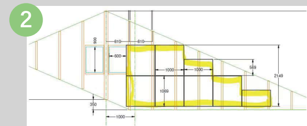
Structural design
